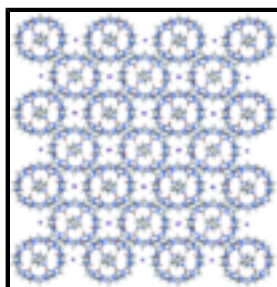
Fig. 3. Illustration of the packing of complex (I) in the bc -plane of the crystal. Color coding: C, gray; H, white; N, blue; O, red; I, purple; H-bonds, red-yellow striped.
